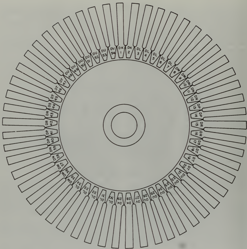
FIGURE 10-62. Typical turbine rotor blade moment-weight distribution.
